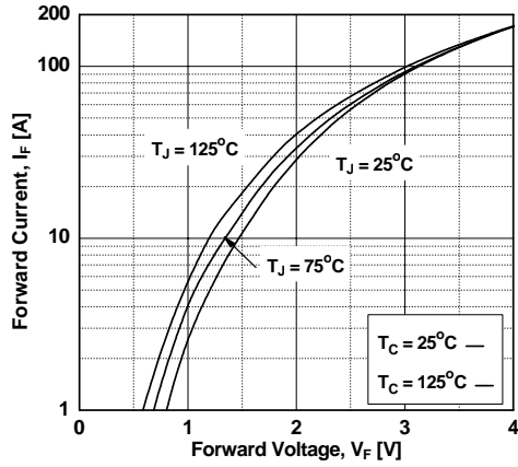
Figure 19. Forward Characteristics
